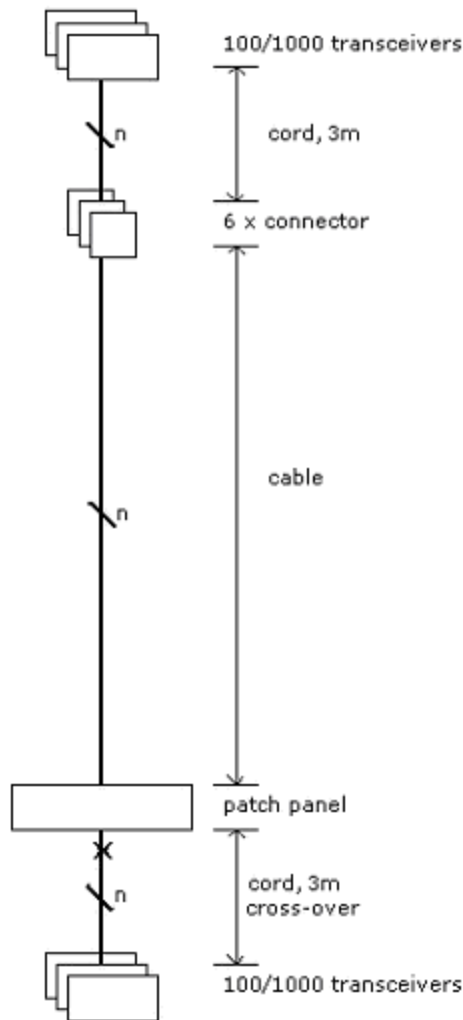
Figure 2-1 Channel Layout
