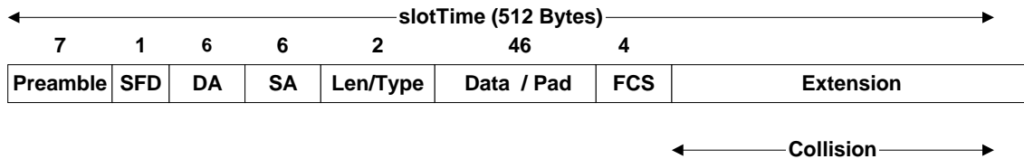
Figure 4 - 9 Collisions during extension within slotTime
