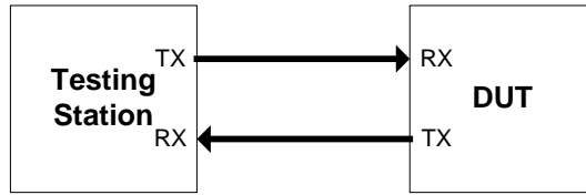
Figure 4 - 22 Test Setup #2 for 100BASE-X Devices
