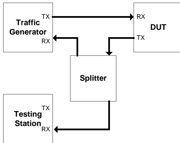
Figure 4 - 23 Test Setup #1 for 1000BASE-X Devices
