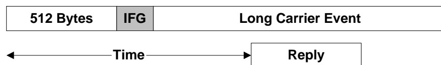
Figure 4 - 5 Does not defer
