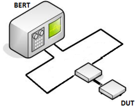
83D.I – 3: Setup used for Group 4: Receiver Electrical Requirements testing
