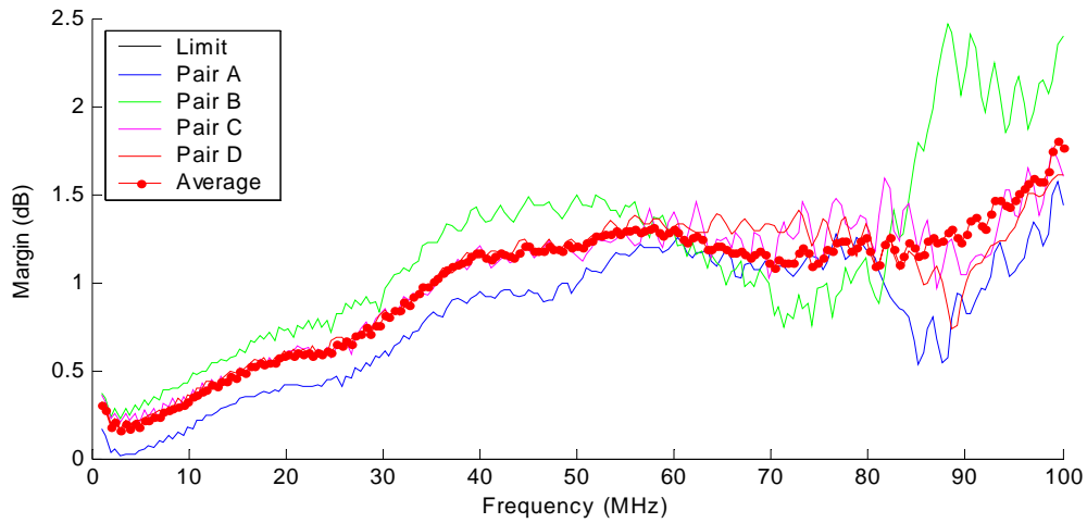
Figure 40.C-2: Attenuation data gathered using Agilent 4395A Network Analyzer
