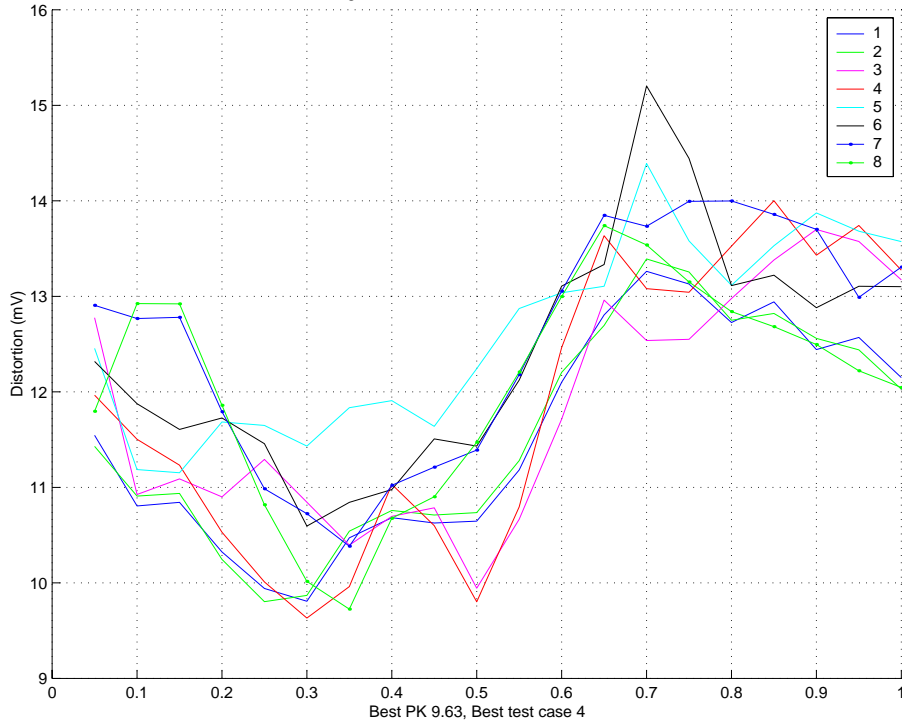
Figure B-29: Distortion Stats for DUT 29
