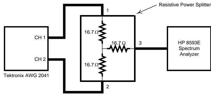
Figure 40.A-9: Test setup for disturbing signal generator linearity measurement
